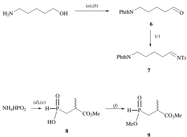
Scheme 3 Synthesis of imine 7 and phosphinic ester 9 . Reagents and conditions: (a), phthalic anhydride, toluene, heat, 99%; (b), i, \text{Me}_2\text{SO} , (\text{COCl})_2 , -78^\circ\text{C} ; ii, \text{NEt}_3 , 91%; (c), \text{Ph}_3\text{CNH}_2 , toluene, heat, 100%; (d), \text{HN}(\text{SiMe}_3)_2 , 110^\circ\text{C} ; (e), \text{H}_2\text{C}=\text{C}(\text{CH}_3)\text{CO}_2\text{Me} , 96% overall; (f), \text{CH}_2\text{N}_2 , \text{Et}_2\text{O} , 100%.
