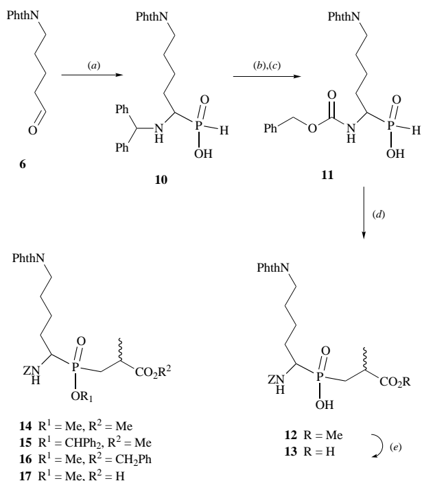
Scheme 4 Synthesis of pseudo-dipeptide phosphinate 13 . Reagents and conditions: (a), \text{H}_3\text{PO}_2 , \text{Ph}_2\text{CHNH}_2 , \text{H}_2\text{O}-\text{EtOH} , 80^\circ\text{C} , 36%; (b), \text{CF}_3\text{CO}_2\text{H} , heat, 85%; (c) \text{PhCH}_2\text{OCOC} , \text{H}_2\text{O} , pH 9–9.5, <5^\circ\text{C} , 100%; (d), i, \text{HN}(\text{SiMe}_3)_2 , 110^\circ\text{C} ; ii, \text{H}_2\text{C}=\text{C}(\text{CH}_3)\text{CO}_2\text{Me} , 94%; (e), i, \text{KOH} , \text{H}_2\text{O} ; ii, 1,1'-carbonyldiimidazole, \text{CH}_2\text{Cl}_2 , 86%.
